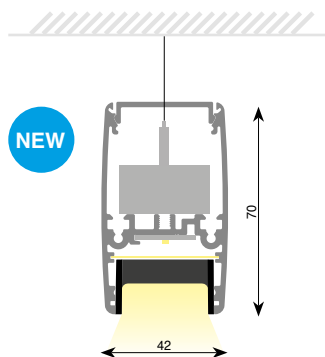
Average weight of equipped profile: 2.8 kg/m
